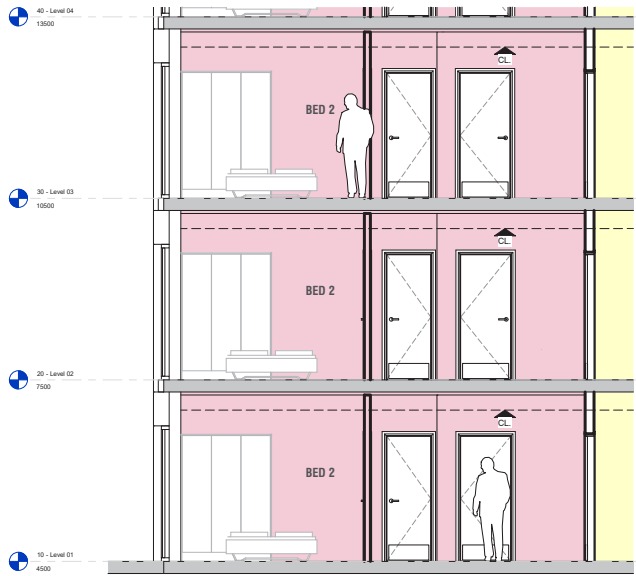
3 Block E Section Detail T8 1 : 50
