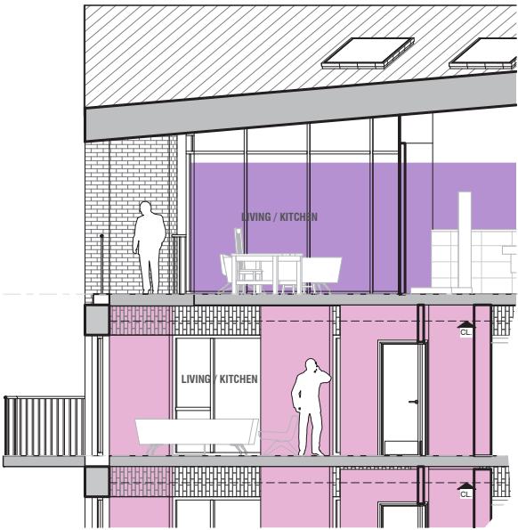
3 Block E Section Detail T7 1 : 50
