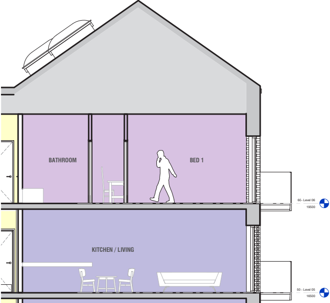
3 Block C - Section Detail T6
