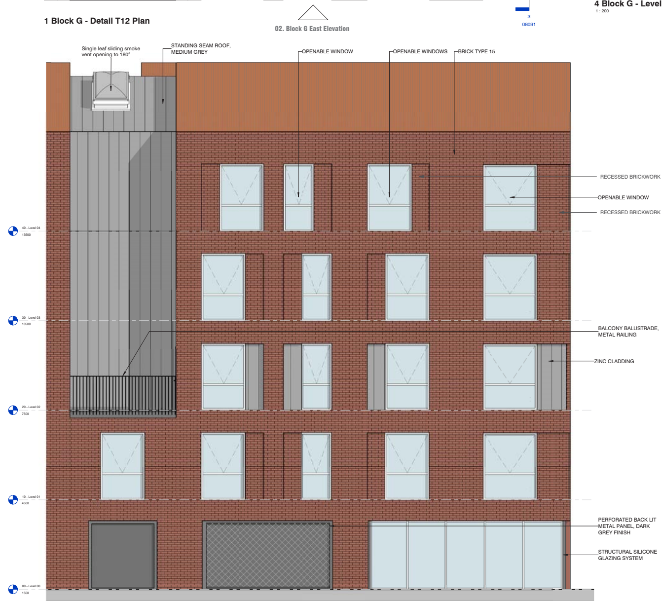
2 Block G East Elevation - Detail T12
