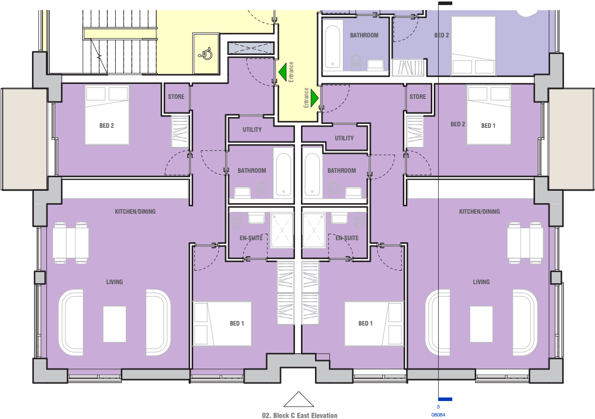
1 Block C - Detail T5 Plan
