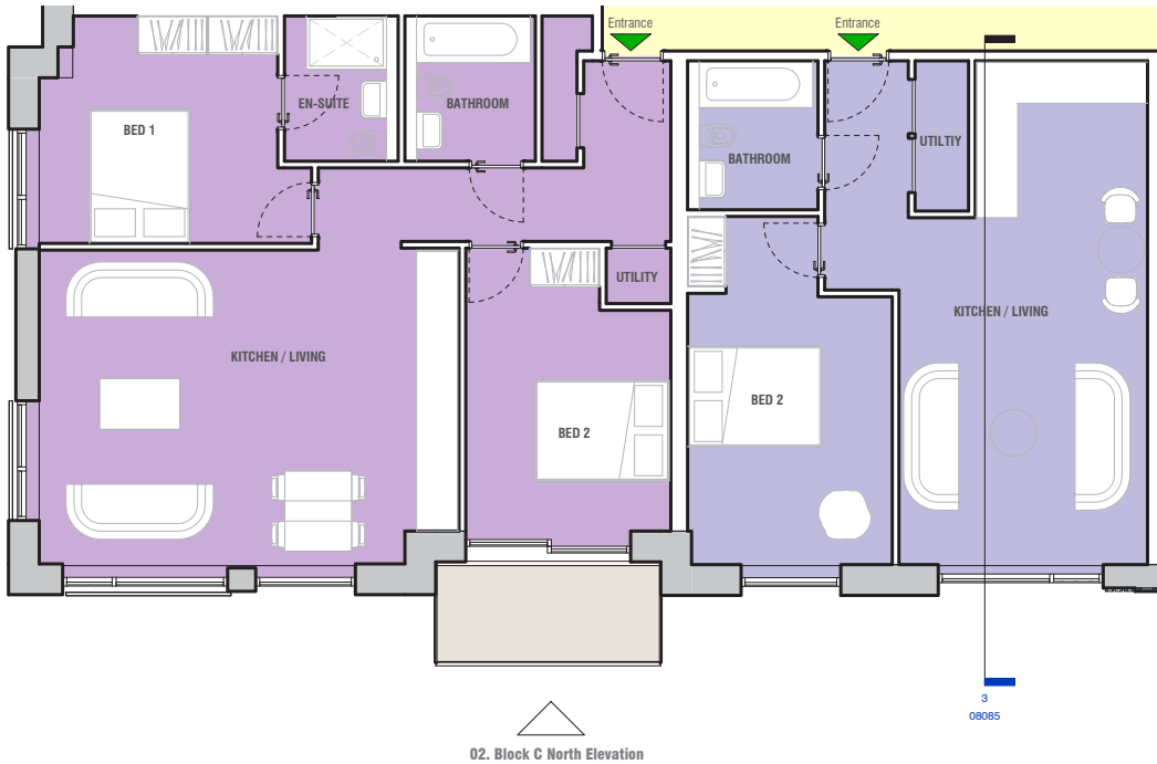
1 Block C - Detail T6 Plan
