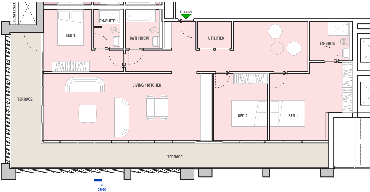
1 Block A-Detail T1 Plan 1:50
