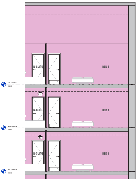
4 Block F - Level 03-05- 1:200
