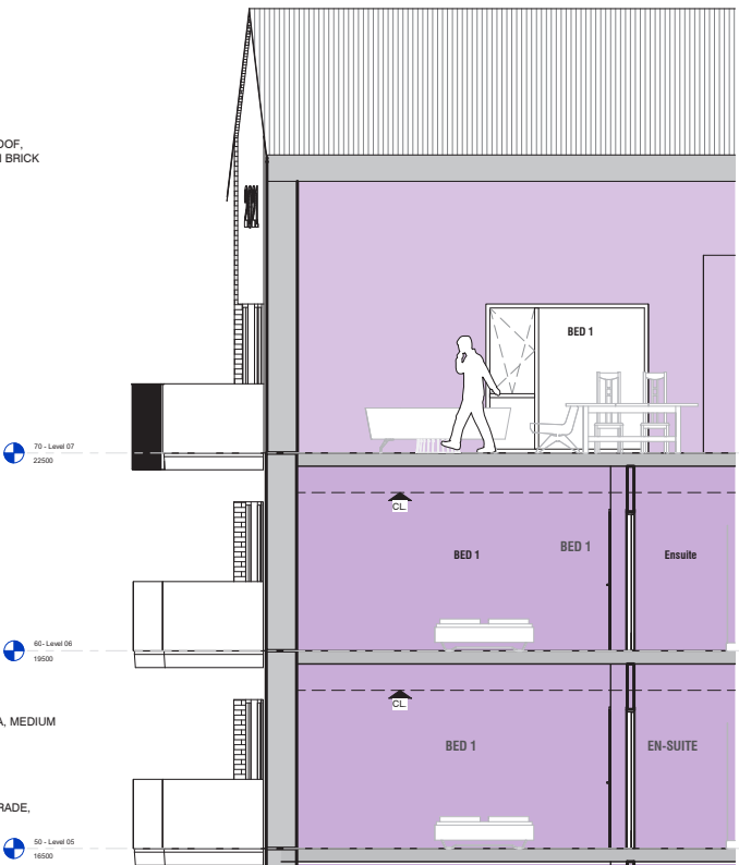
3 Block D - Section Detail T4
