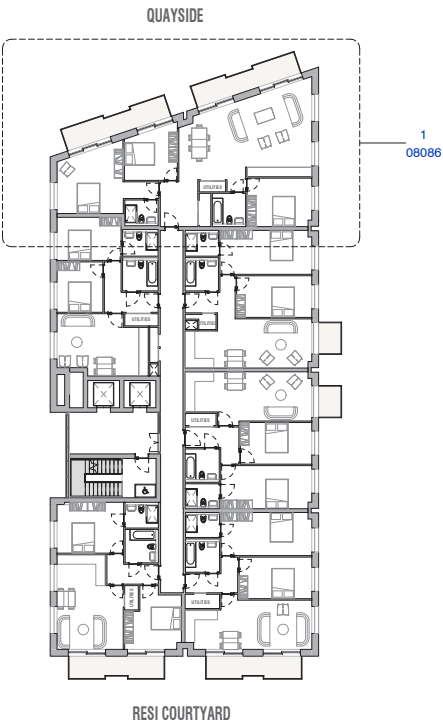
4 Block E- Level 6 1 : 200
