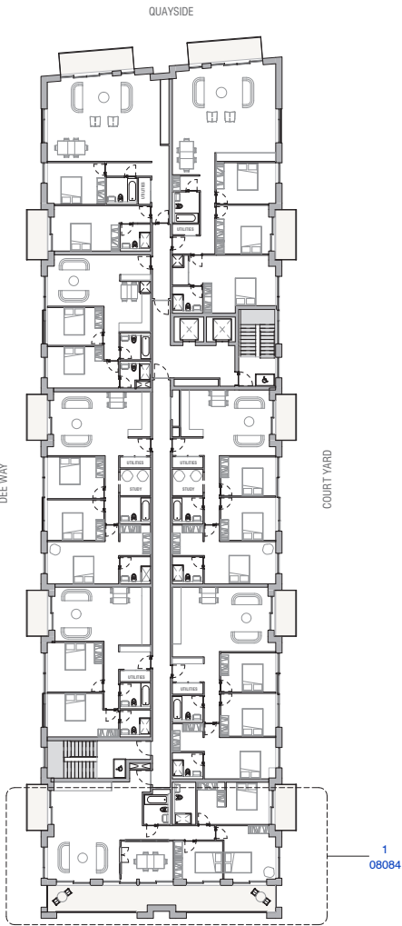
4 Block C - Level 08 Penthouse
