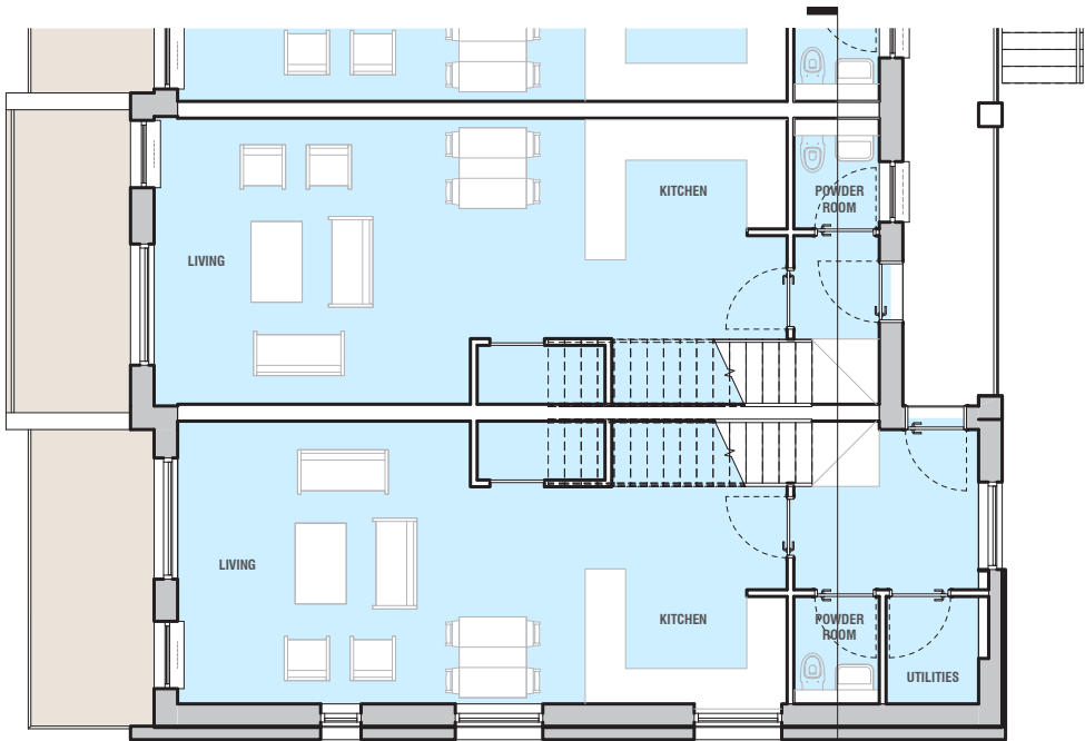
1 Block H1 - Detail T14 Plan
