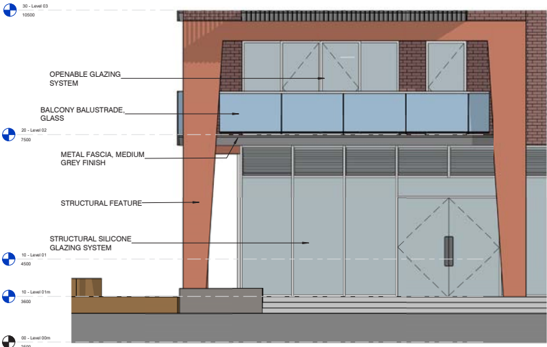
2 Block C West Elevation - Detail T3
