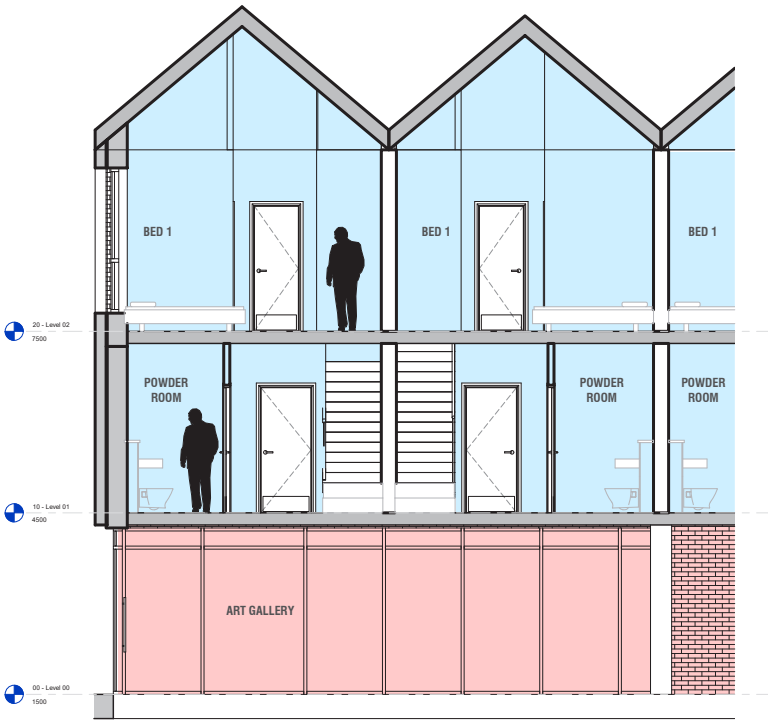
3 Block H1 Section Detail T14
