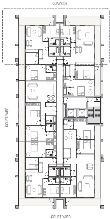
4 Block B- Level 10 1:200
