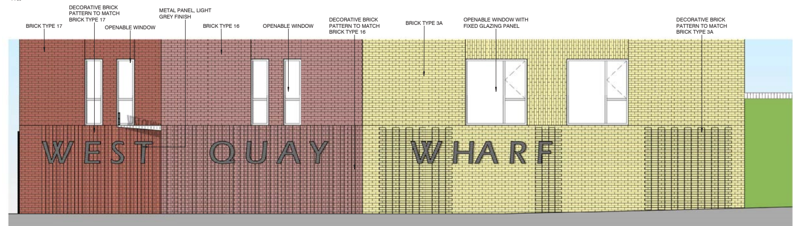
2 Block H2 West Elevation - Detail T16 1:50
